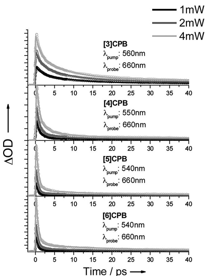
Figure 4. Pump-power-dependent TA decay profile of [n]\text{CPB} oligomers in toluene.
