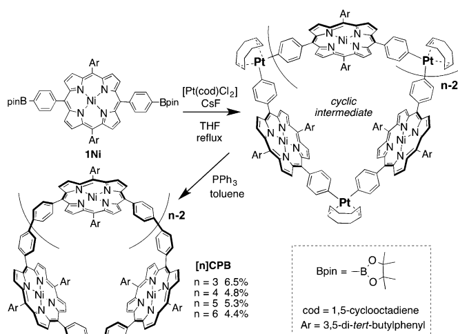
Scheme 2. Synthesis of [n]CPB oligomers.
